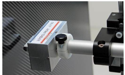
Fig. 3: Lamb wave measurement on a sandwich component
