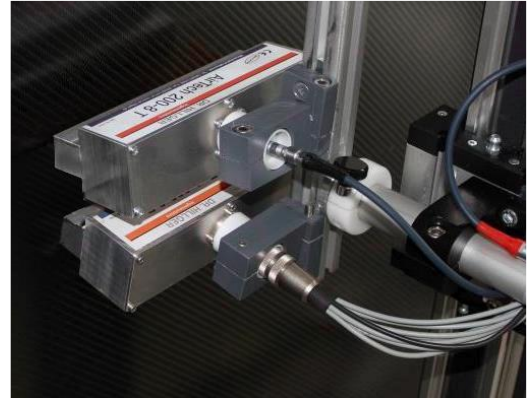
Fig. 2: One-sided investigation with V-arrangement of the probe arrays
