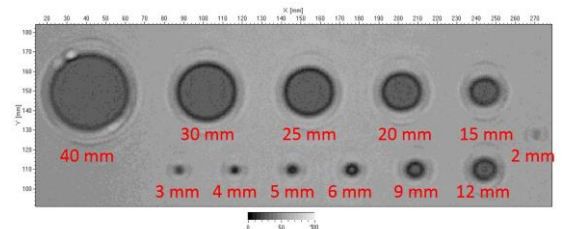
Fig. 4: C-scan of flat bottom holes in a 5,3 mm CFRP plate with 300 kHz testing frequency
