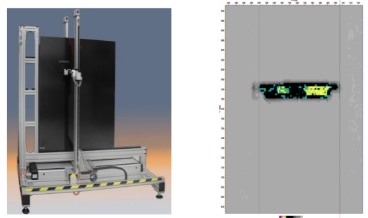
Fig. 5: Testing of a CFRP plate with the FlatScan 1000, artificial defect is shown in a C-scan
